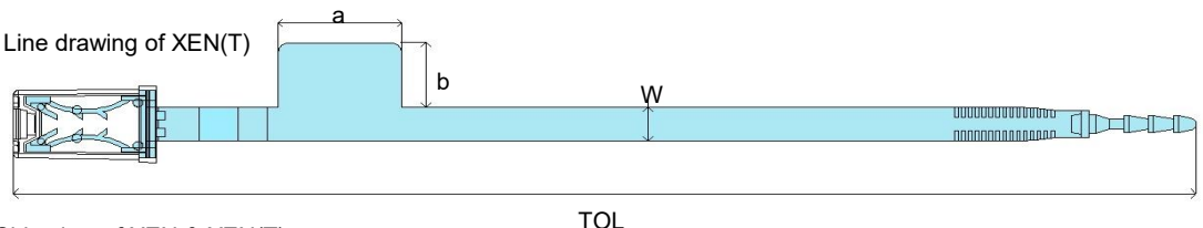
Fig 3: Side view of XEN & XEN(T)
